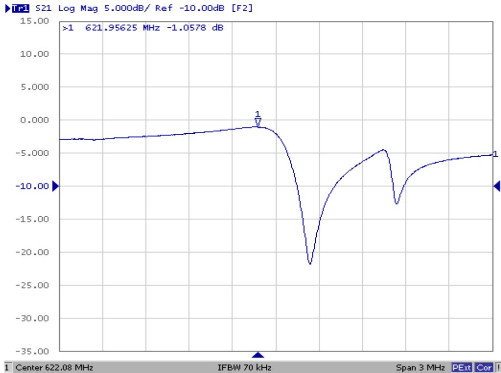
Frequency Response
