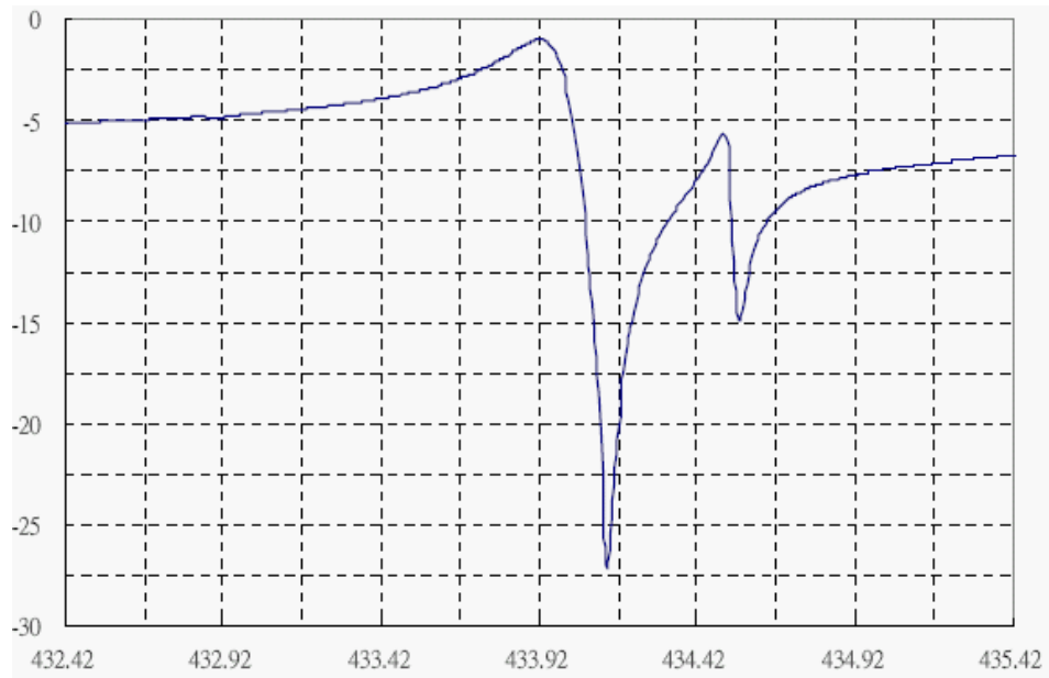
Frequency Response
