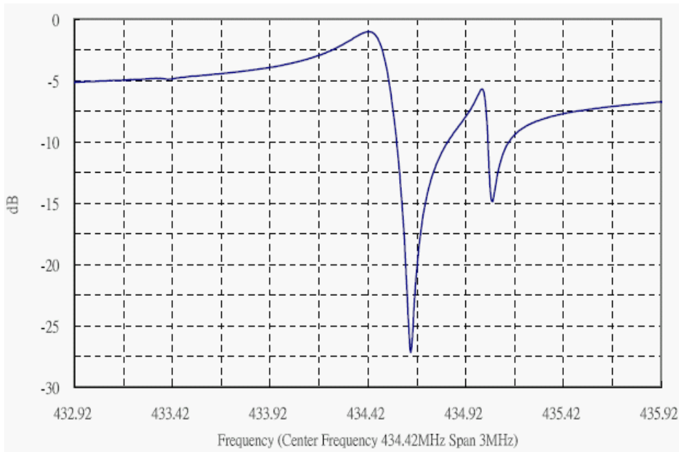
Frequency Response
